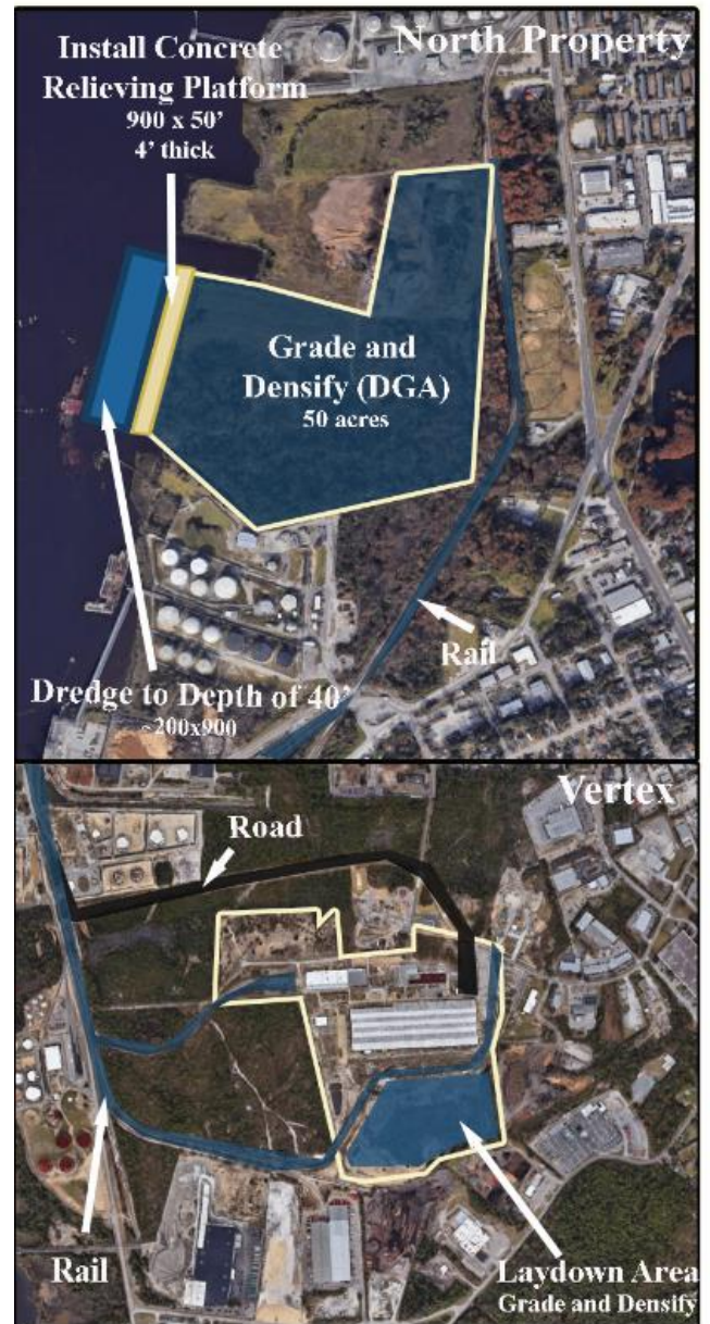
Figure 38 Integrated scenario for two properties, detailed view.
