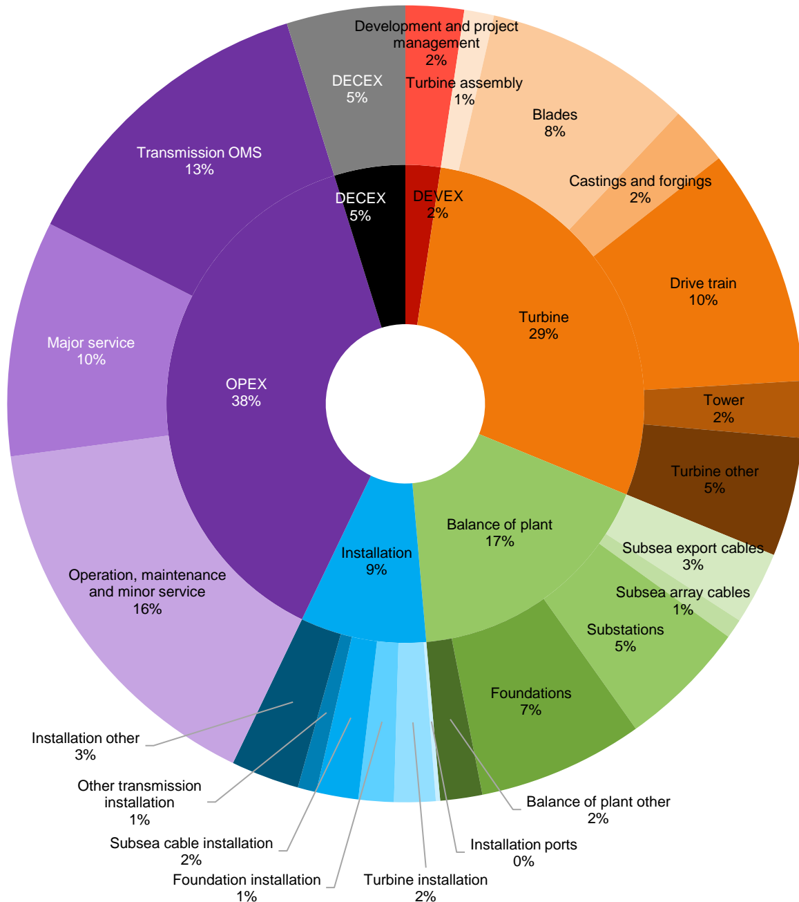
Figure 5 CAPEX and OPEX for an OSW farm of 1,000 MW installed capacity using 15 MW turbines.
