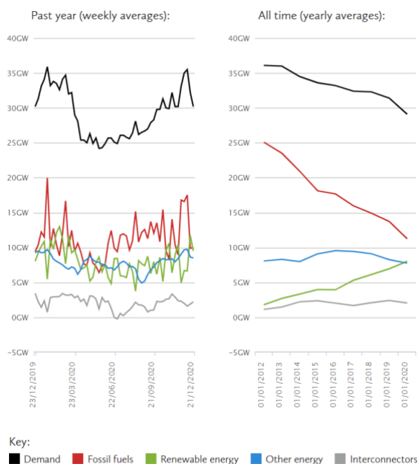
Figure 3 The UK electricity generation mix.
