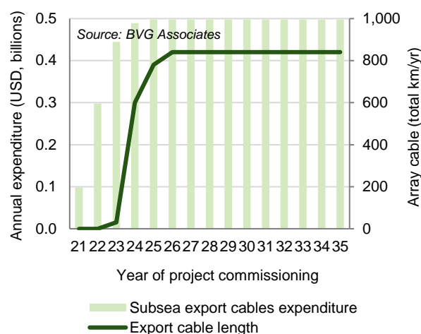
Figure 16 Demand and expenditure for export cable, shown versus year of project commissioning.
