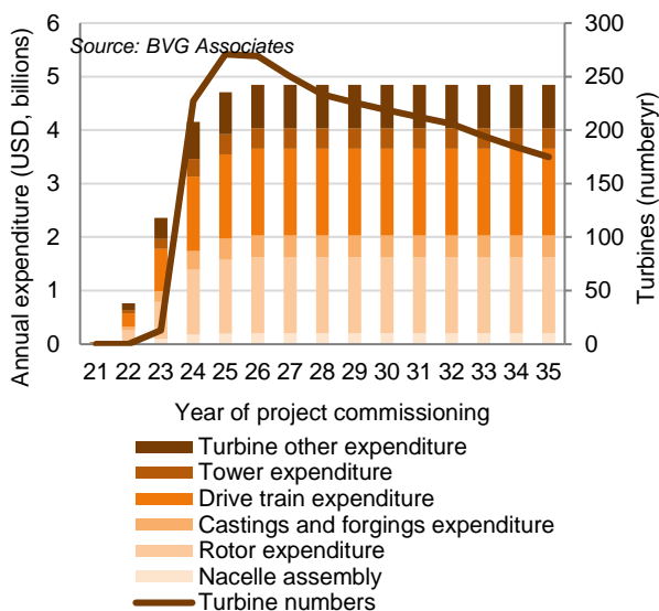
Figure 12 Demand and expenditure for turbines, shown versus year of project commissioning.
