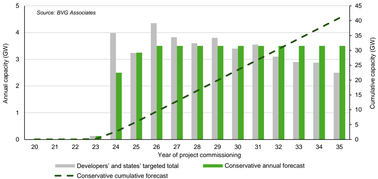
Figure 2 Conservative forecast of US East Coast installed capacity.
