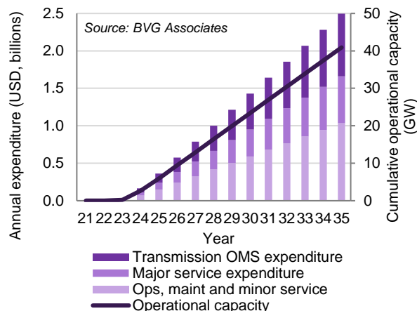
Figure 20 Demand and expenditure for OMS, shown versus year of project commissioning.
