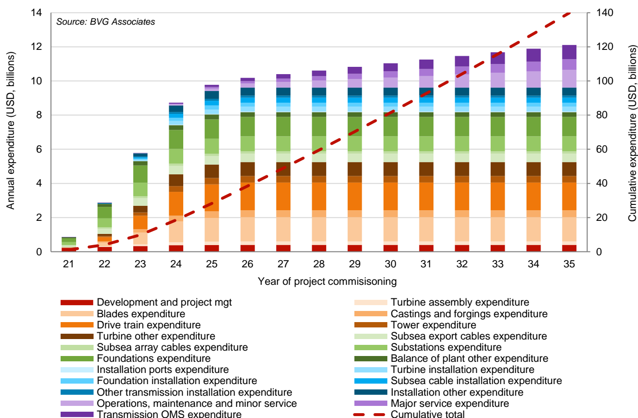
Figure 4 Forecast of annual OW expenditure.
