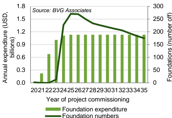
Figure 15 Demand and expenditure for foundations, shown versus year of project commissioning.
