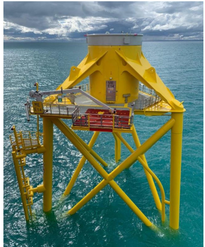
Figure 14 A typical jacket foundation for an OSW turbine at Moray East.
