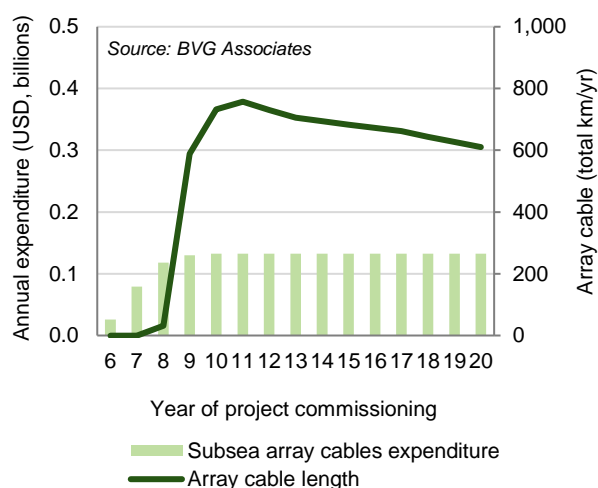
Figure 17 Demand and expenditure for array cable, shown versus year of project commissioning.
