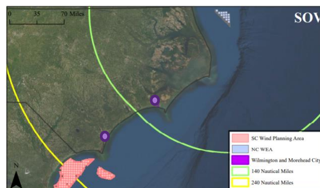
Figure 27 Map of North Carolina WEA and Suitable SOV Distances.
